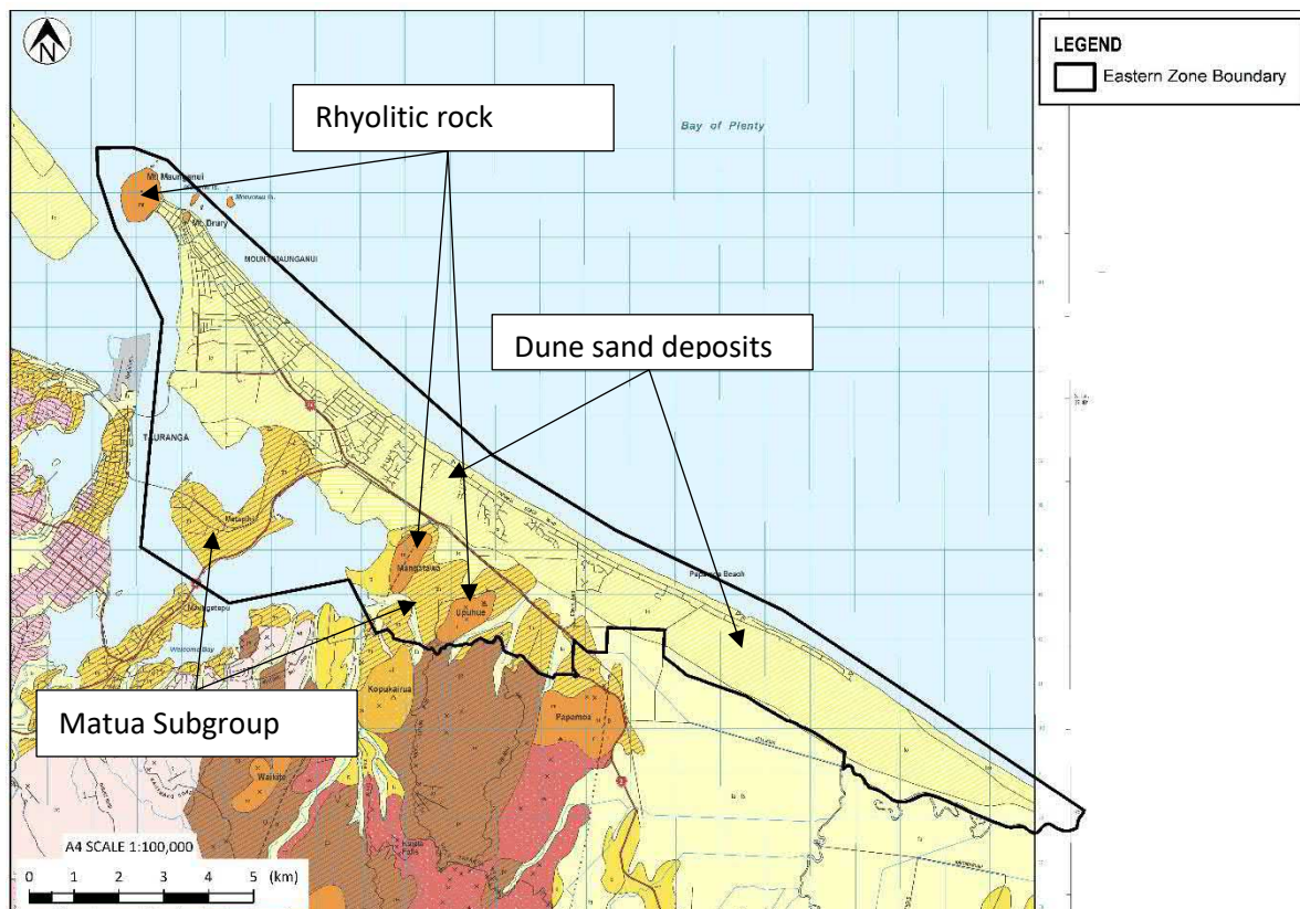
Figure 3.4: Eastern Zone overlain on the Briggs et al (1996) geological map - note as shown on the figure a small portion of the Eastern Zone is not included in the figure. This was mapped in the QMAP geological map series (2010) and in Briggs et al . (2006)
