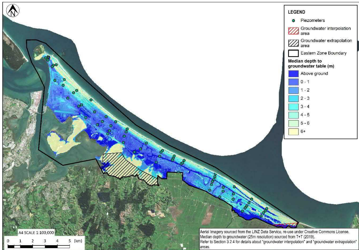
Figure 3.8: Groundwater 1.25m shallower than current day median depth to groundwater model
