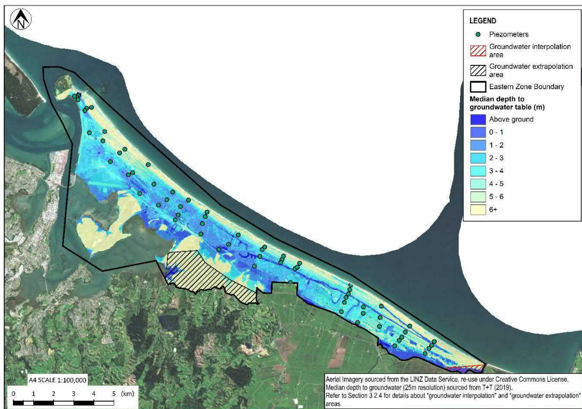
Figure 3.7: Current day median depth to groundwater model
