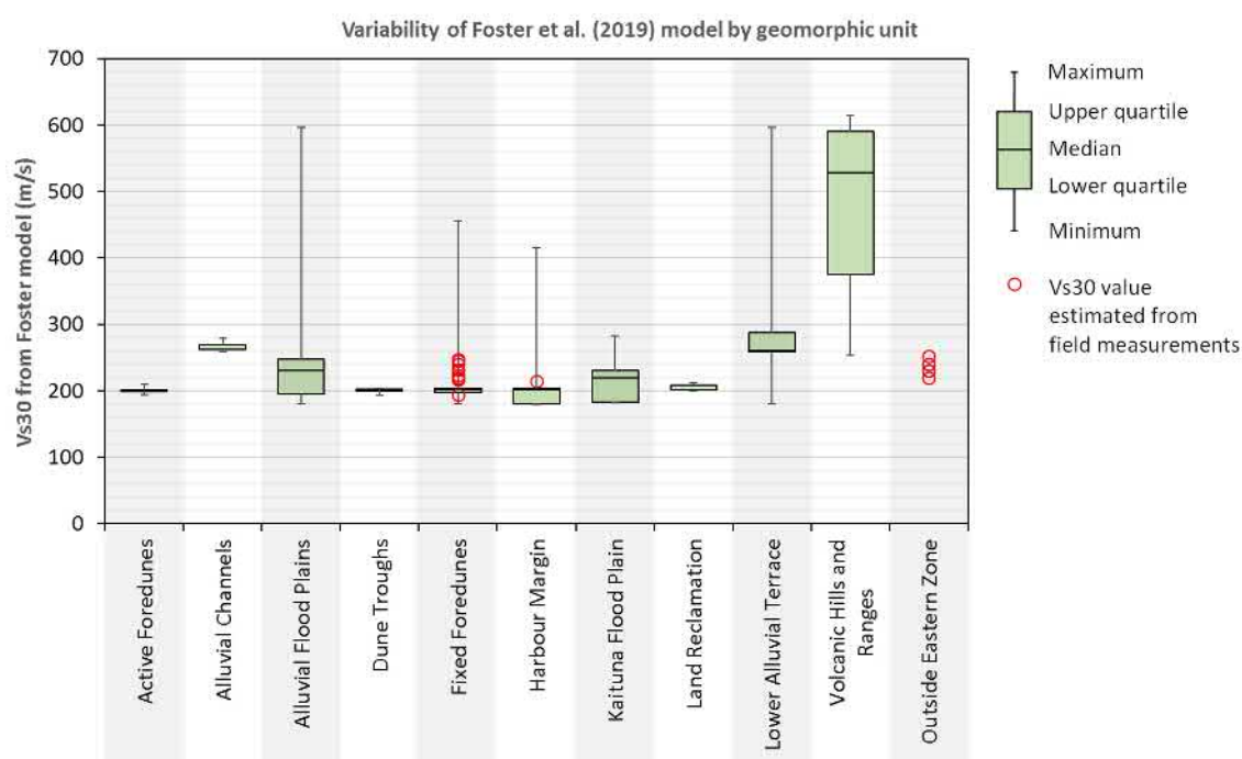
Figure 4.11: Variability of Foster et al. (2019) model Vs30 values by geomorphic terrain
