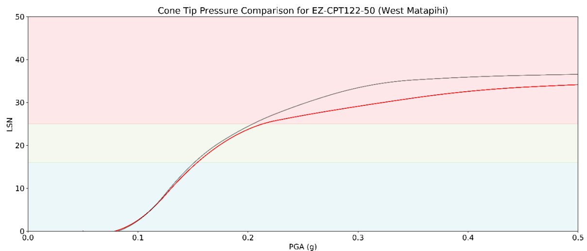
Figure 4.7: PGA vs. LSN plots from adjacent 50 MPa (red) and 100 MPa (grey) tip resistance cones (location two) in the Matapihi Harbour Margin geomorphic terrain for an assumed groundwater depth of 1 m
