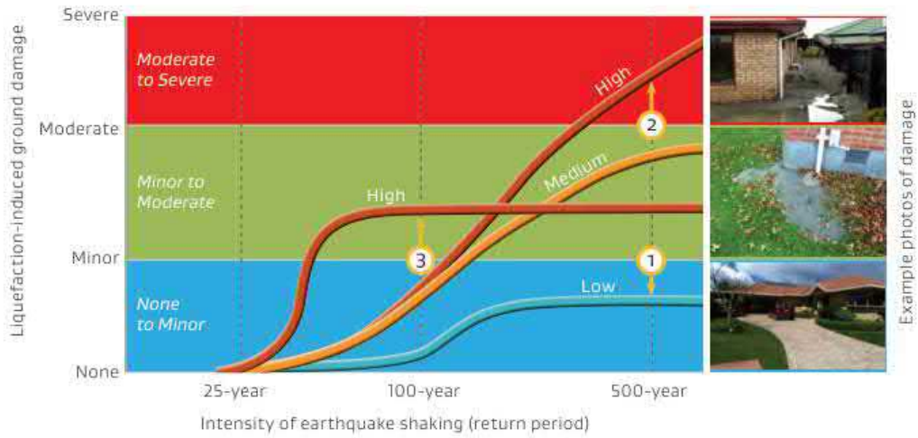
Figure 4.25: Example ground damage response curves for low, medium, and high liquefaction vulnerability categories, and performance criteria used for liquefaction categorisation - from MBIE/MfE Guidance (2017)
