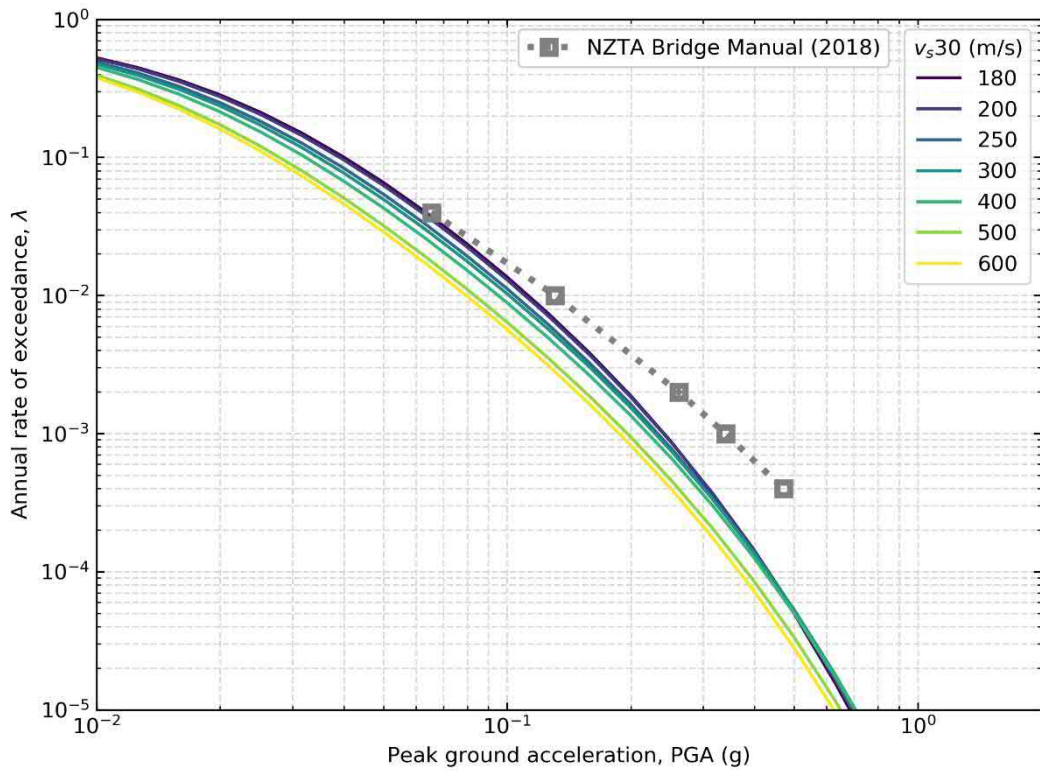
Figure 3.11: Seismic hazard curves for peak ground acceleration (PGA) from BSL (2019) illustrating the effect of soil conditions as quantified through Vs30. The hazard curves using the NZTA Bridge Manual (2018) methodology for site subsoil class D are also provided for reference
