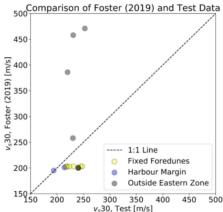
Figure 4.10: Comparison of Vs30 values from Foster et al. (2019) model and estimated from field measurements
