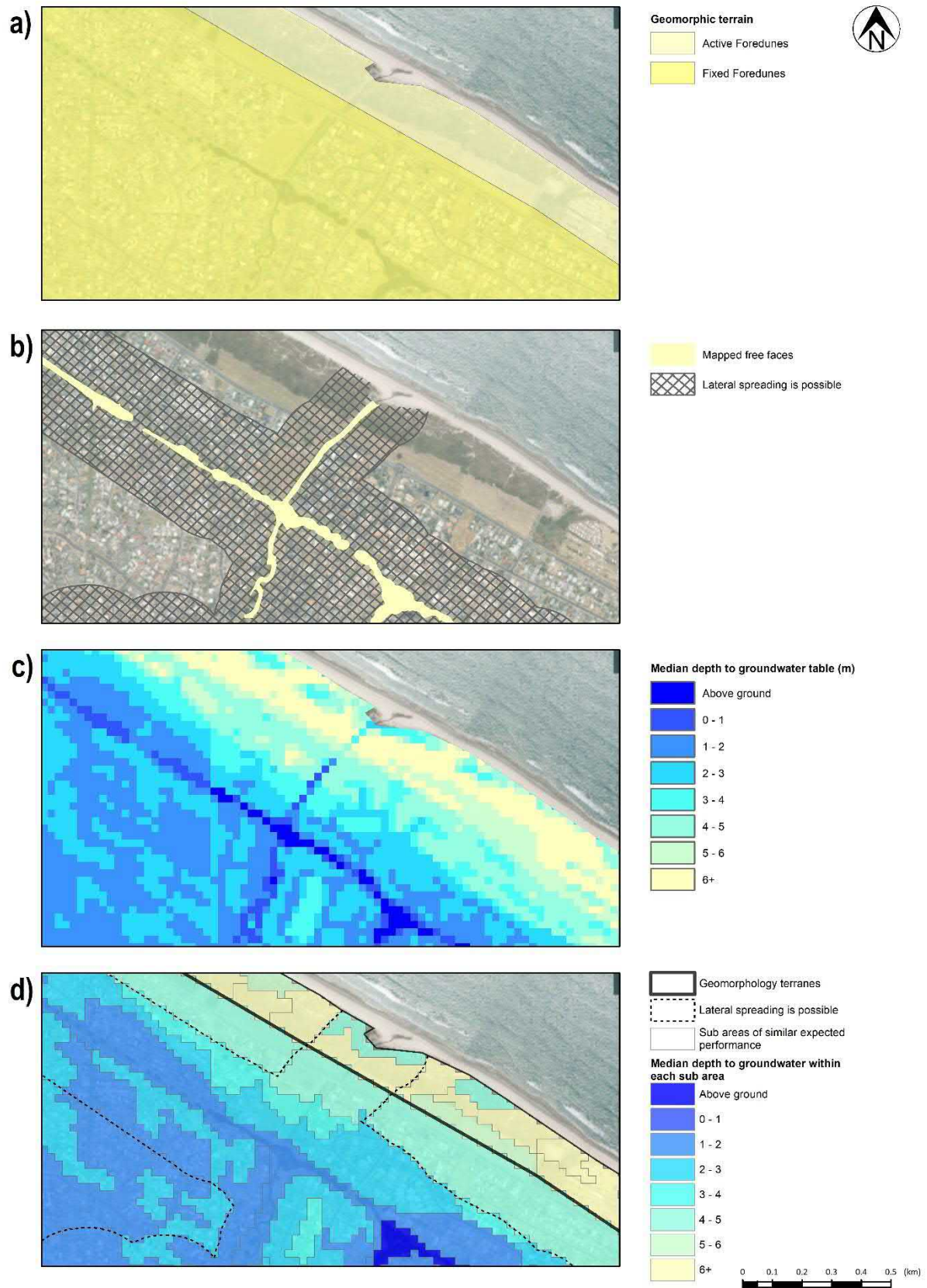
Figure 4.19: Portion of the Eastern Zone showing: a) geomorphic terrain boundaries; b) lateral spreading is possible buffer zone; c) median depth to groundwater model; and d) sub areas of similar expected performance derived from a), b) and c).
