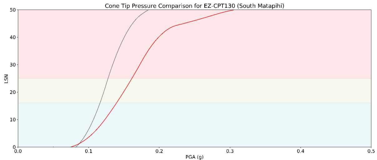
Figure 4.6: PGA vs. LSN plots from adjacent 50 MPa (red) and 100 MPa (grey) tip resistance cones (location one) in the Matapihi Harbour Margin geomorphic terrain for an assumed groundwater depth of 1 m
