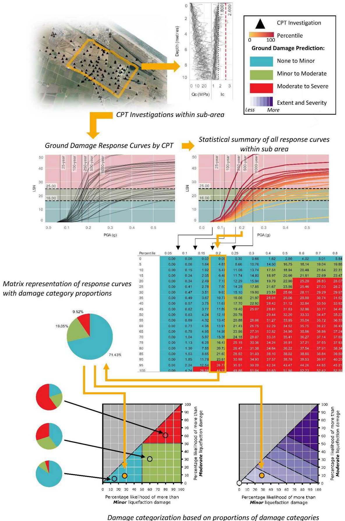
Figure 4.21: Methodology used to represent land damage using the analytical model for the Eastern Zone
