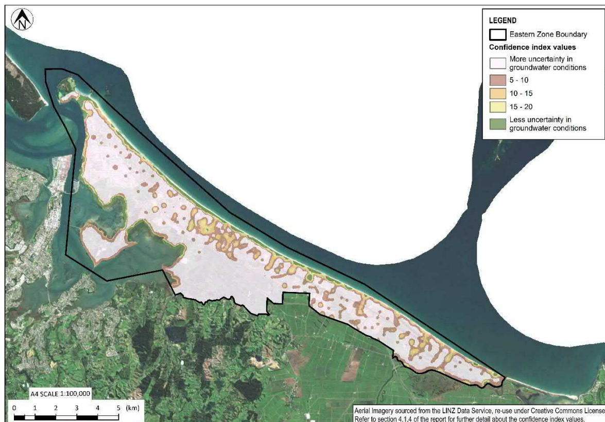
Figure 4.9: Confidence index value map for Tauranga. A higher index value represents higher confidence in the groundwater model, a lower confidence index value represents lower confidence in the groundwater model
