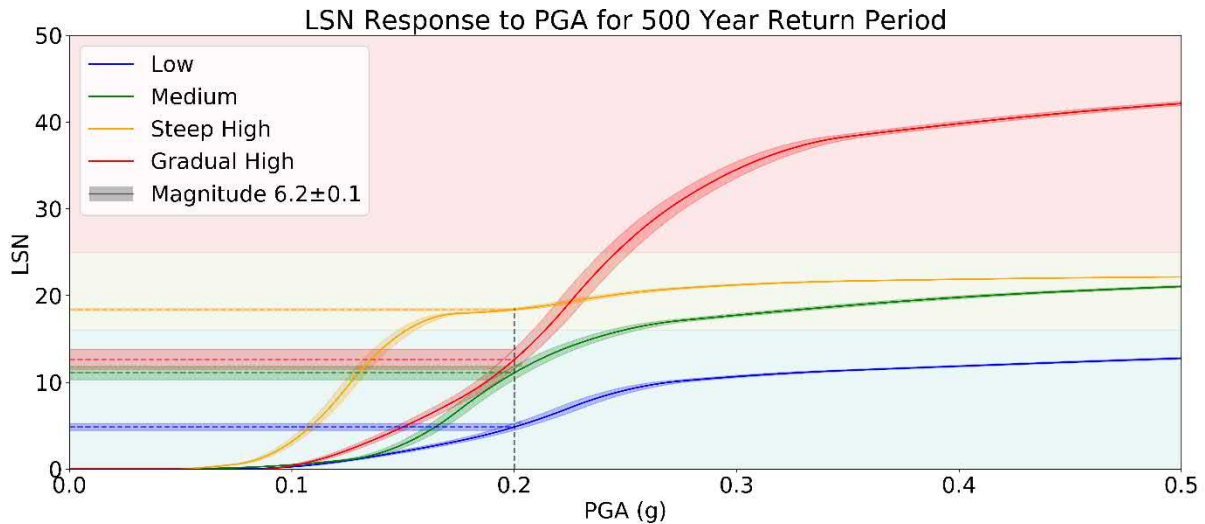
Figure 4.13: Effect of variation in magnitude on liquefaction consequences for four different ground damage response curves (assuming a magnitude 6.2 earthquake and probability of liquefaction of P_L = 15\% ). The buffered area shows the variation in LSN for magnitude 6.2 \pm 0.1 (i.e. magnitude 6.1 to 6.3). The vertical line shows the PGA value of 0.20 g for the 500 year design event. The horizontal lines show the corresponding LSN values for each of the four ground damage response curves. Higher LSN values indicate a higher likelihood of more severe liquefaction consequences. The width of the buffered area provides an indication of how sensitive the predicted ground damage is to variations in the magnitude for that particular response curve (also refer to Table 4.5).
