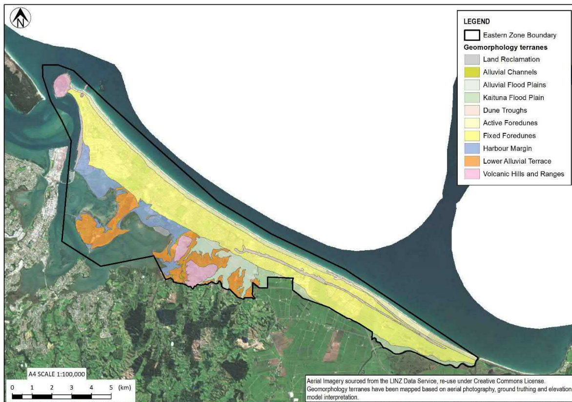
Figure 3.5: Geomorphic map of the Eastern Zone
