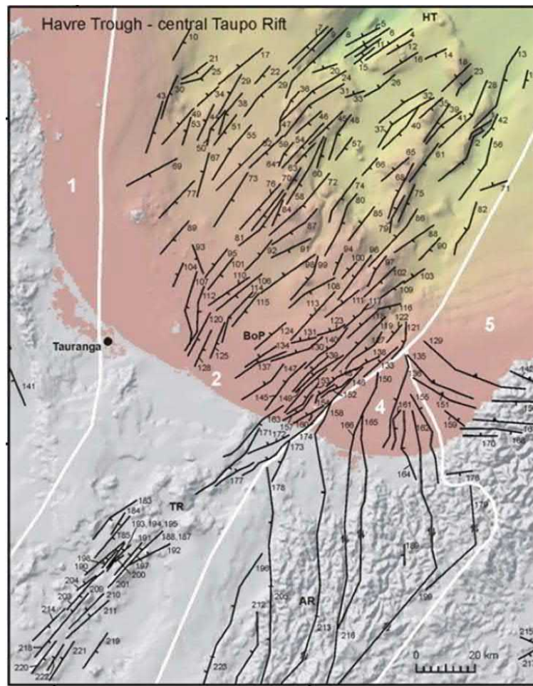
Figure 3.9: Active faults in the Bay of Plenty and Taupo Rift. The fault sources are shown as black lines and Area 2, which is bounded by the white lines, identifies the Bay of Plenty and Taupo Rift
