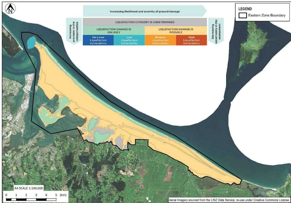
Figure 4.27: Liquefaction vulnerability categories for Tauranga City assigned in this study. Refer to Figure 4.26 for map legend
