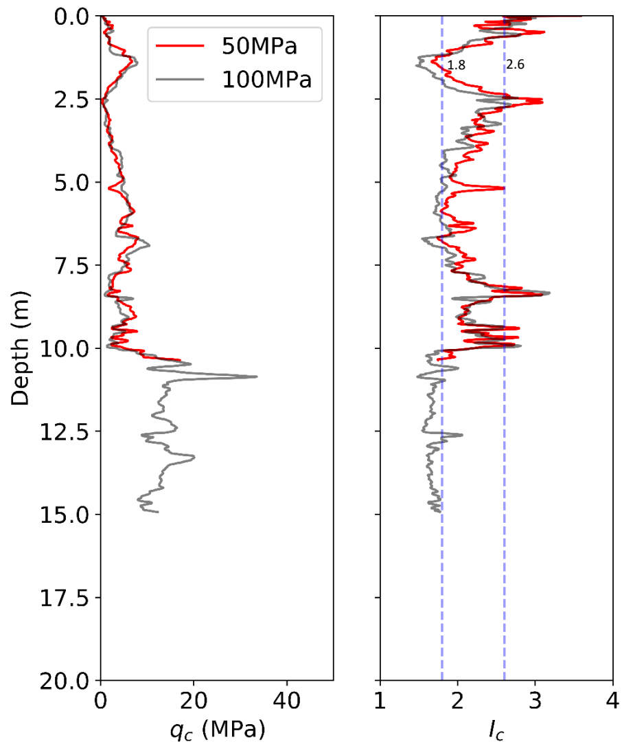
Figure 4.4: CPT cone tip density ( q_c ) vs. depth and soil behaviour type ( I_c ) vs. depth from adjacent 50 MPa and 100 MPa tip resistance cones (location one) in the Matapihi Harbour Margin geomorphic terrain
