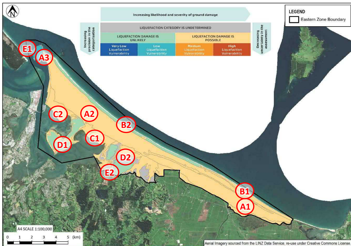
Figure 5.3: Liquefaction vulnerability categories for Tauranga City assigned in this study. Refer to Figure 4.26 for map legend
