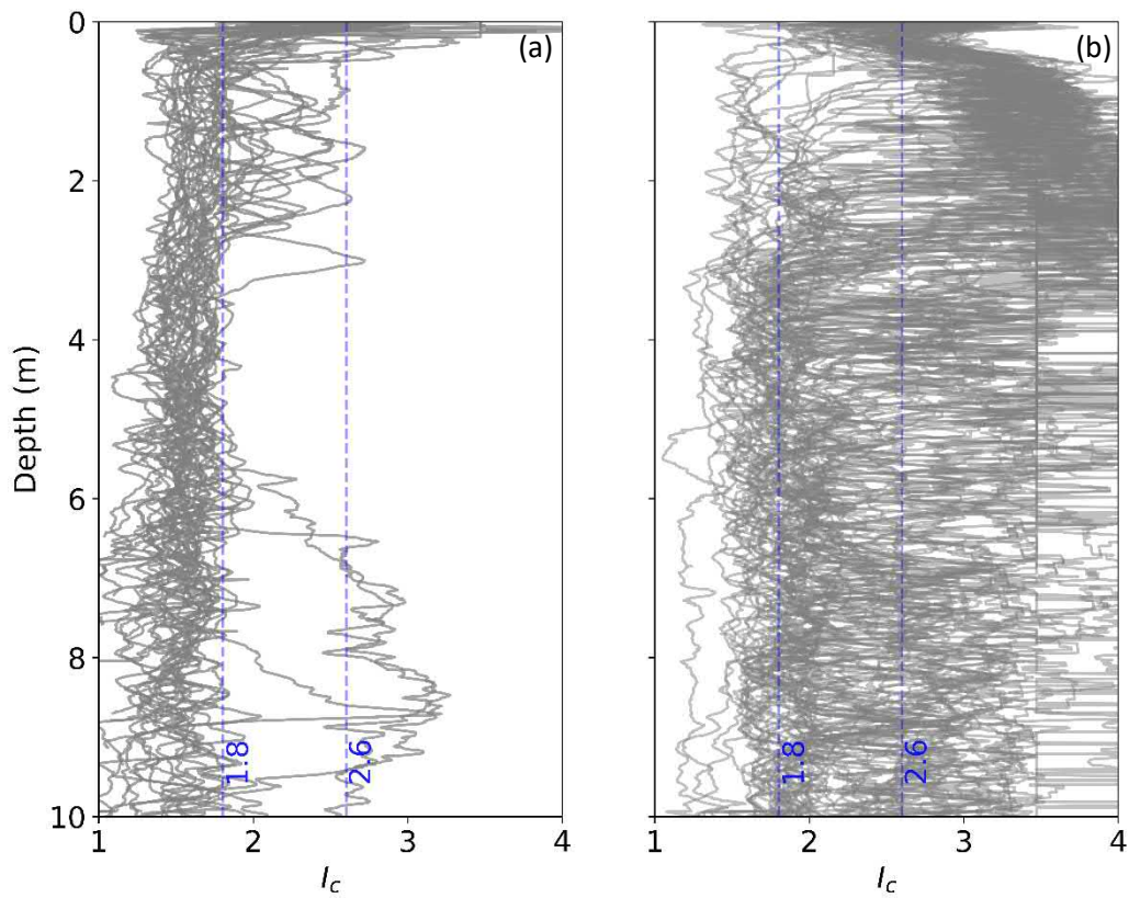
Figure 4.2: CPT soil behaviour type ( I_c ) vs. depth from (a) Active Foredune and (b) Kaituna Flood Plain
