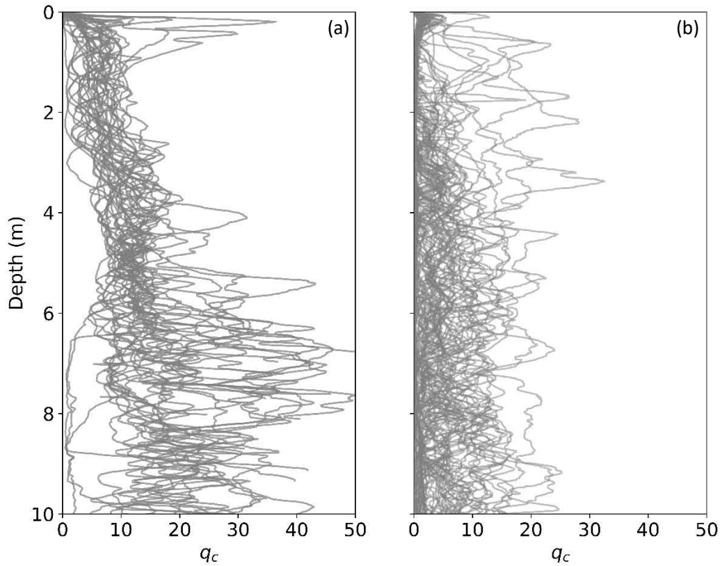
Figure 4.1: CPT cone tip density ( q_c ) vs. depth from the (a) Active Foredune and (b) Kaituna Flood Plain
