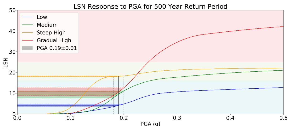
Figure 4.12: Effect of variation in PGA on liquefaction consequences for four different ground damage response curves (assuming a magnitude 6.2 earthquake and probability of liquefaction of P_L = 15\% ). The vertical lines show the indicative range in PGA values of 0.18 to 0.20 g for the 500 year design event (from Table 4.3). The horizontal lines show the corresponding LSN values for each of the four ground damage response curves. Higher LSN values indicate a higher likelihood of more severe liquefaction consequences. The distance between horizontal lines of the same colour provides an indication of how sensitive the predicted ground damage is to variations in the PGA value for that particular response curve.
