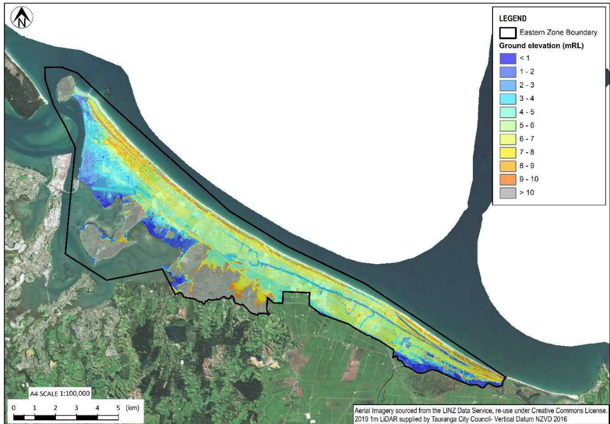
Figure 3.3: Ground surface elevation over the Eastern Zone as represented by the 2019 LiDAR Survey
