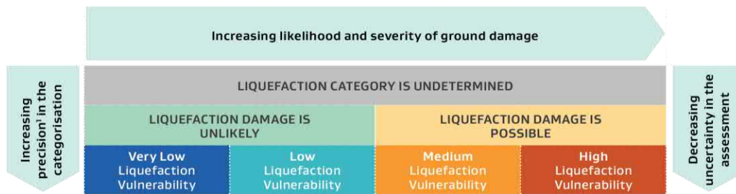
Figure 4.26: Liquefaction vulnerability categories – from MBIE/MfE Guidance (2017)
