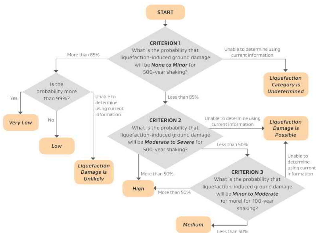
Figure 4.24: Flow chart for determining the liquefaction vulnerability category - from MBIE/MfE Guidance (2017)
